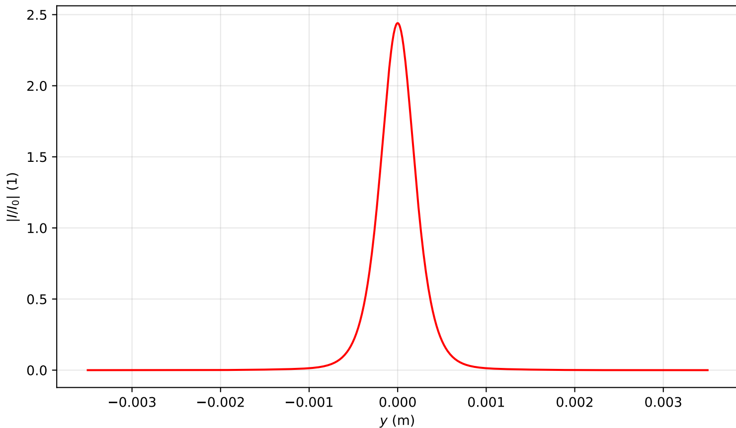
Intensity profile I(x=0, y, z=2.627)/I_0 , \text{Pin}=1.0\text{Pcr} , artificial time
